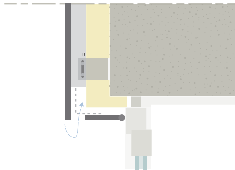
Figure 15: Window Cill
