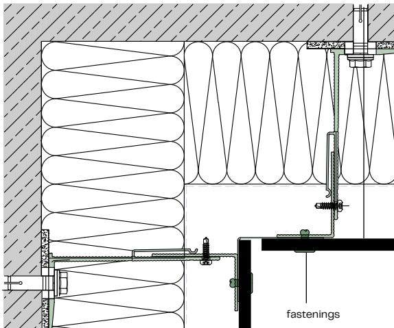
Inner corner A106
