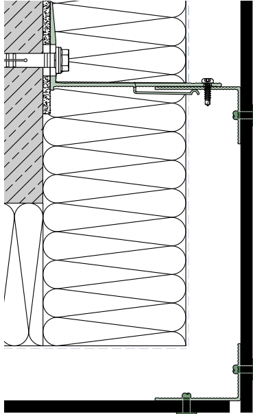
External corner A105
