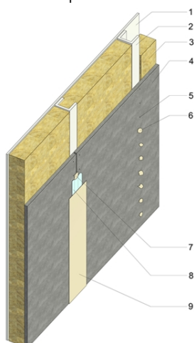
Diagram 1 - typical construction detail with joint filler and mesh tape
