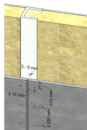
Diagram 3 - typical detail of fixing layout
