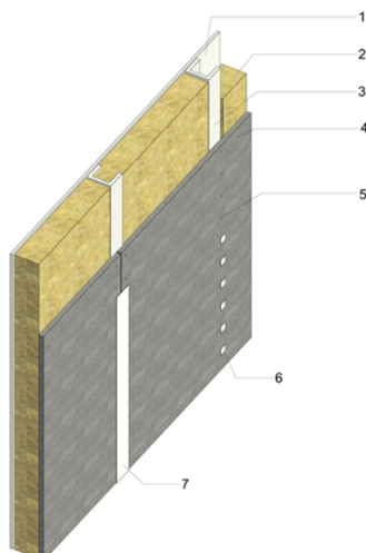
Diagram 2 - typical construction detail with tape
